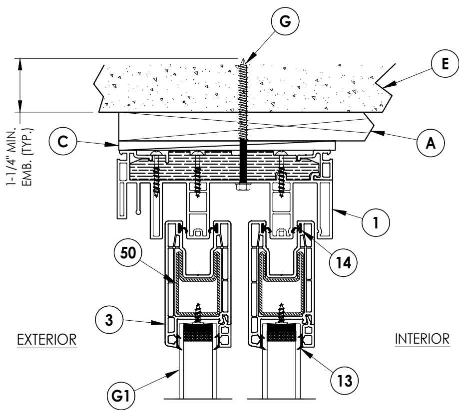
2 VERTICAL CROSS SECTION 3 Shown w/ 1X Buck
