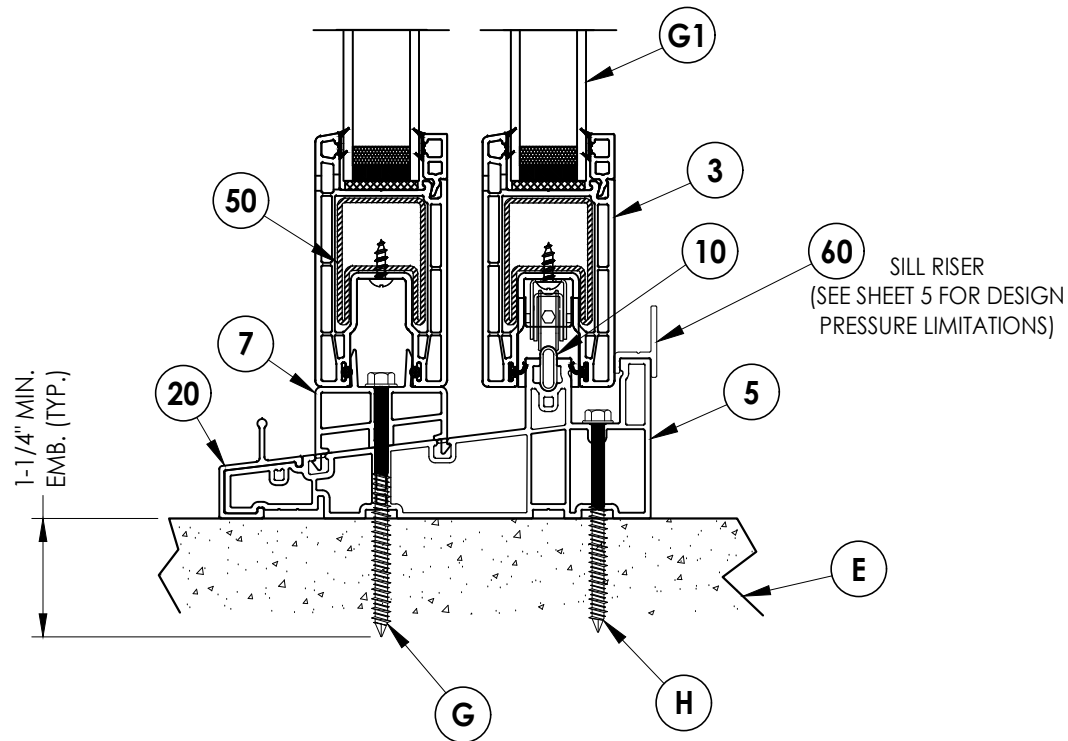
1 VERTICAL CROSS SECTION 3 Shown w/ 2X Buck & Head & Direct to Masonry @ Sill
