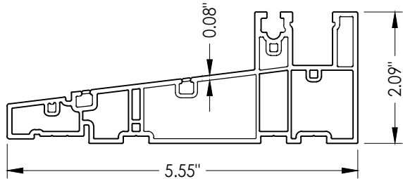
5 FRAME SILL
